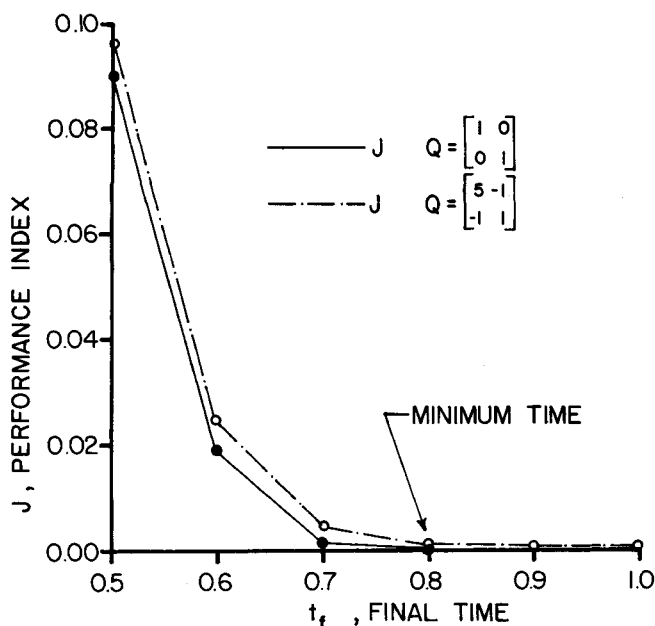
Fig. 1. Performance index vs. final time for system 1 with two different weighting matrices: suboptimal bang-bang control.
