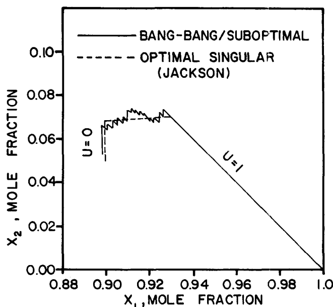
Fig. 8. Computed phase plane for the catalyst blending problem: pure bang-bang control and singular bang-bang control by Jackson (1968).
