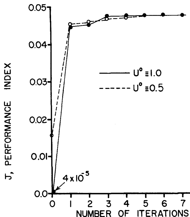
Fig. 9. Performance index versus number of iterations for the catalyst blending problem: pure bang-bang control.
