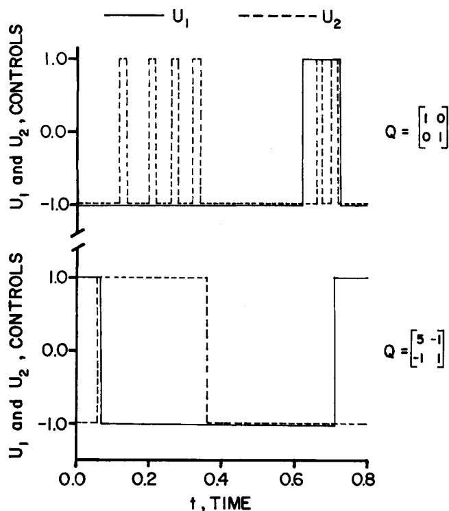
Fig. 3. Computed suboptimal bang-bang control trajectories for system 1 with final time t_f = 0.8 and two different weighting matrices.
