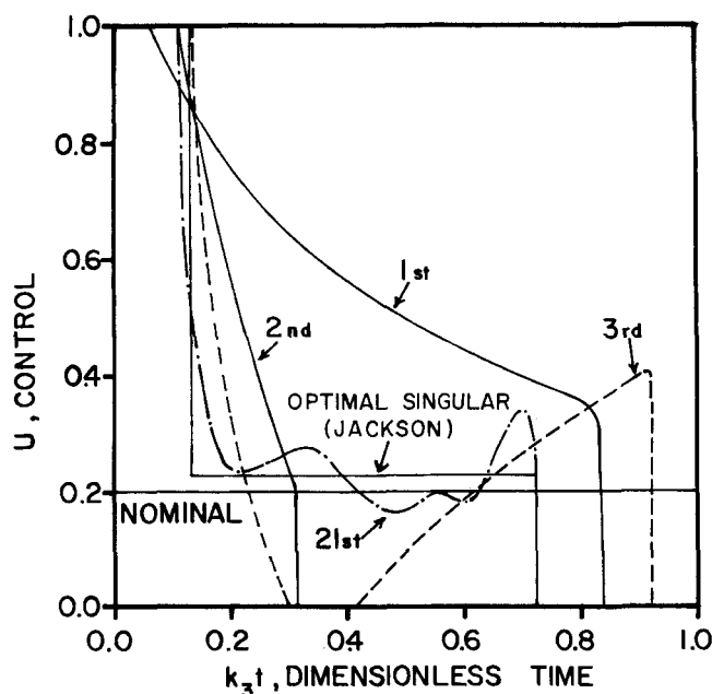
Fig. 7. Computed catalyst blending fraction u vs. dimensionless time (reactor length) in successive number of iterations for the catalyst blending problem: singular bang-bang control.
