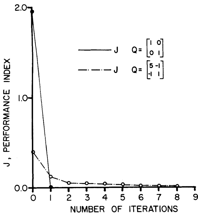
Fig. 2. Performance index vs. number of iterations for system 1 with final time t_f = 0.8 and two different weighting matrices: suboptimal bang-bang control.
