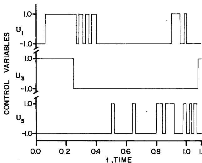
Fig. 6. Computed suboptimal bang-bang control trajectories for system 3 with t_f = 1.10 .
