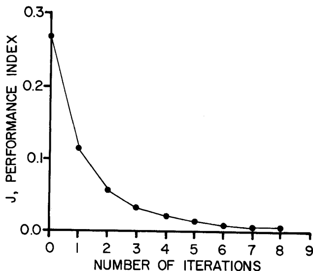
Fig. 4. Performance index vs. number of iteration for system 3 with final time t_f = 1.10 : suboptimal bang-bang control.
