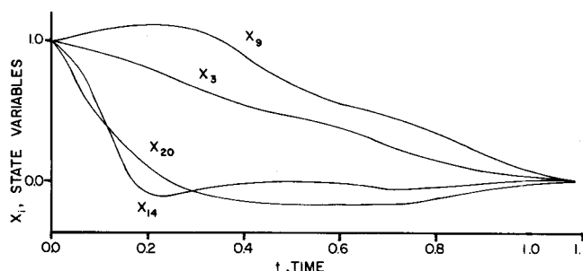
Fig. 5. Computed state trajectories for system 3 with final time t_f = 1.10 : suboptimal bang-bang control.
